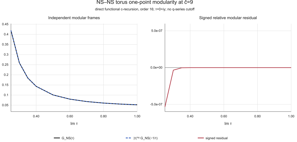
Figure 3: Ordinary NS-NS modular covariance on the imaginary axis. The black curve is the directly evaluated \mathcal{G}_{NS}(iy) ; the dashed blue curve is the independently evaluated and transformed-back y^{-2d}\mathcal{G}_{NS}(i/y) . Their signed relative difference is shown on the right. Both traces use \xi = +1 , so this is a fixed-spin NS-NS comparison and contains neither a (-1)^F insertion nor a hidden Ramond sewing.
